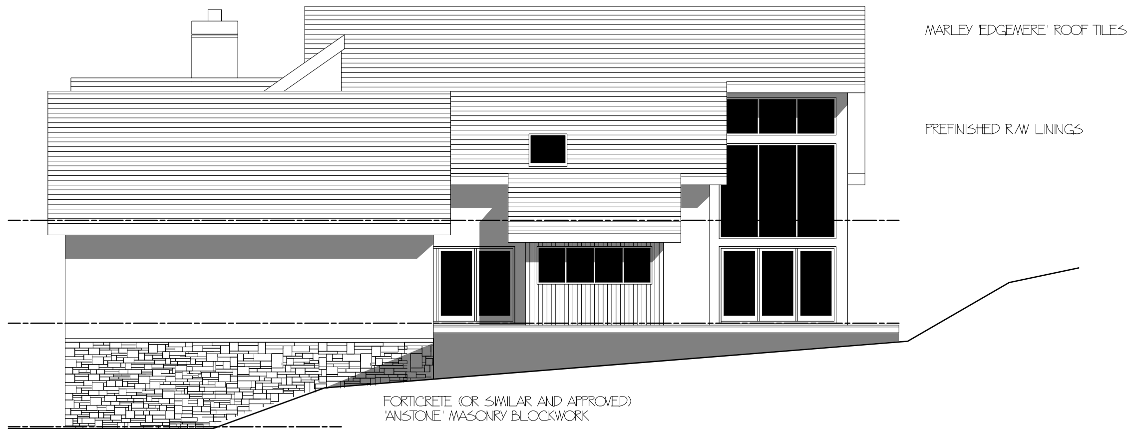
WEST ELEVATION
